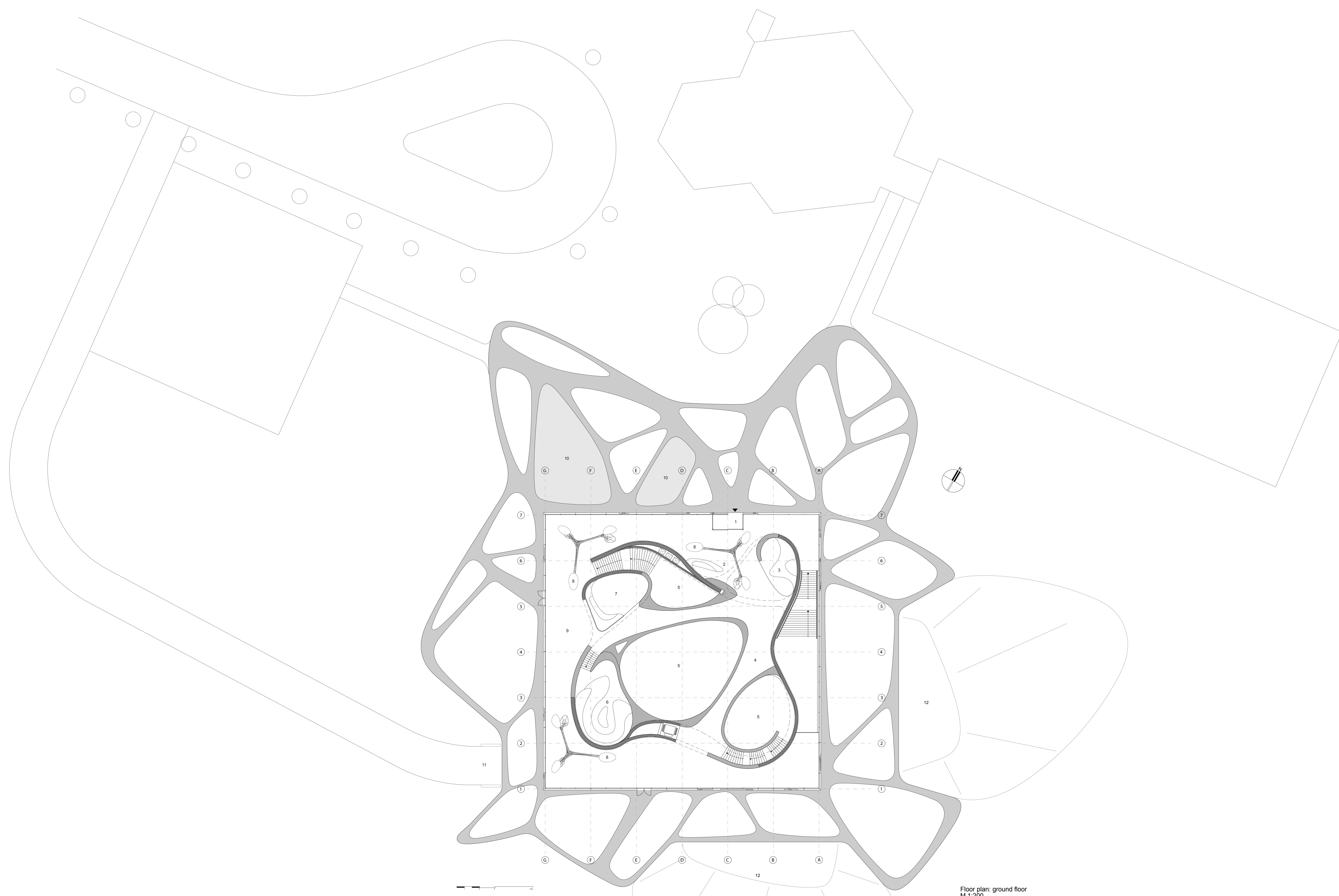
Floor plan: ground floor M 1:200
