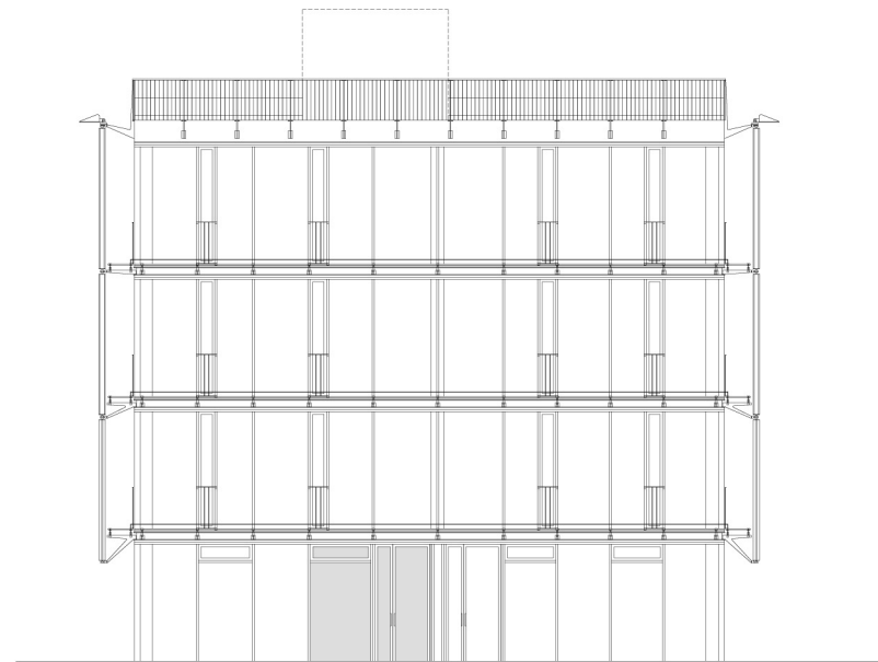
NORTH ELEVATION 1/200
