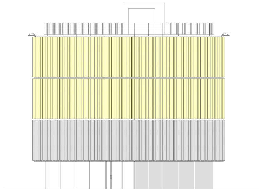
SOUTH ELEVATION 1/200
