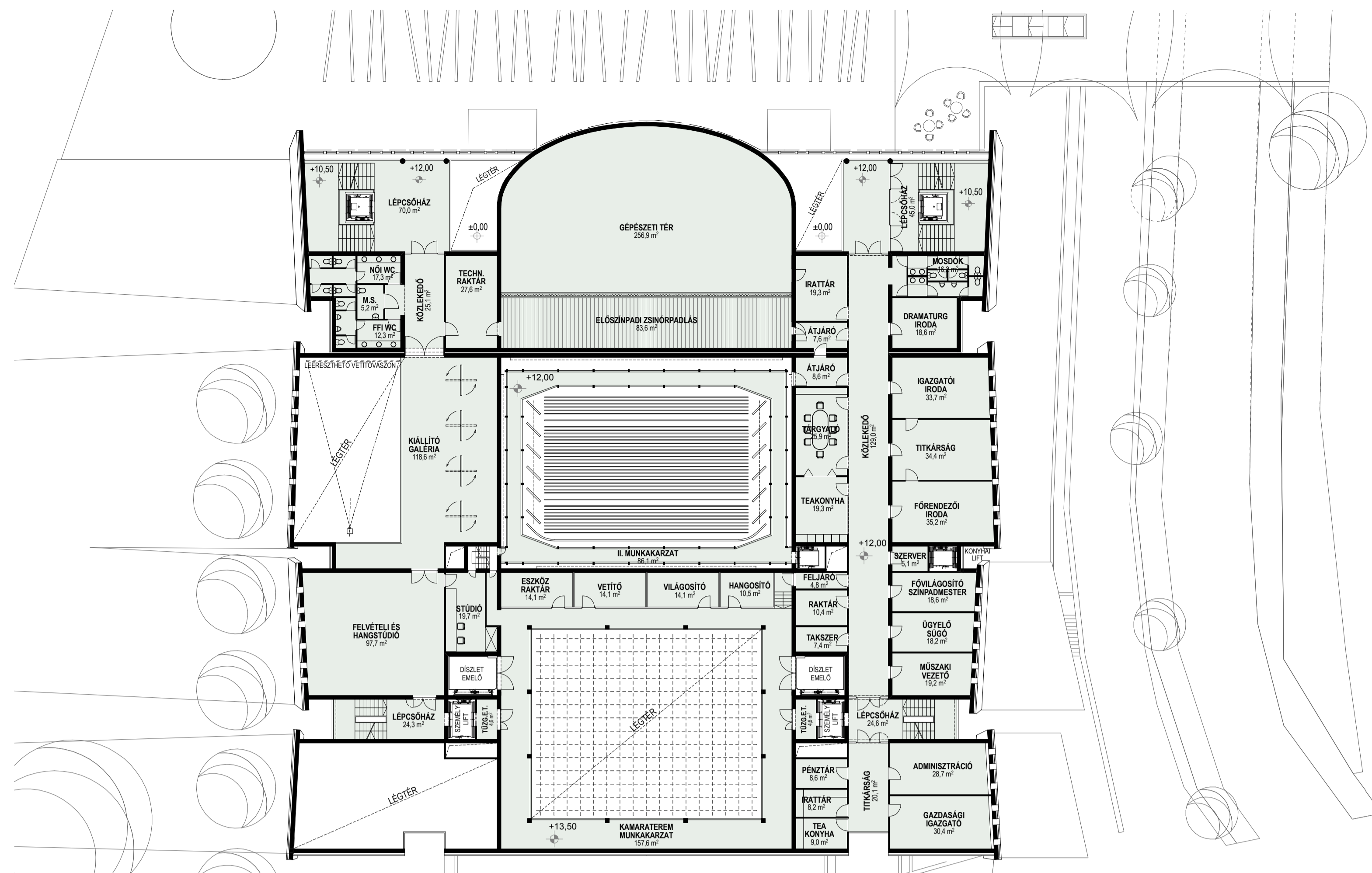
IV. EMELETI ALAPRAJZ +12,00/+13,50m M=1:250
