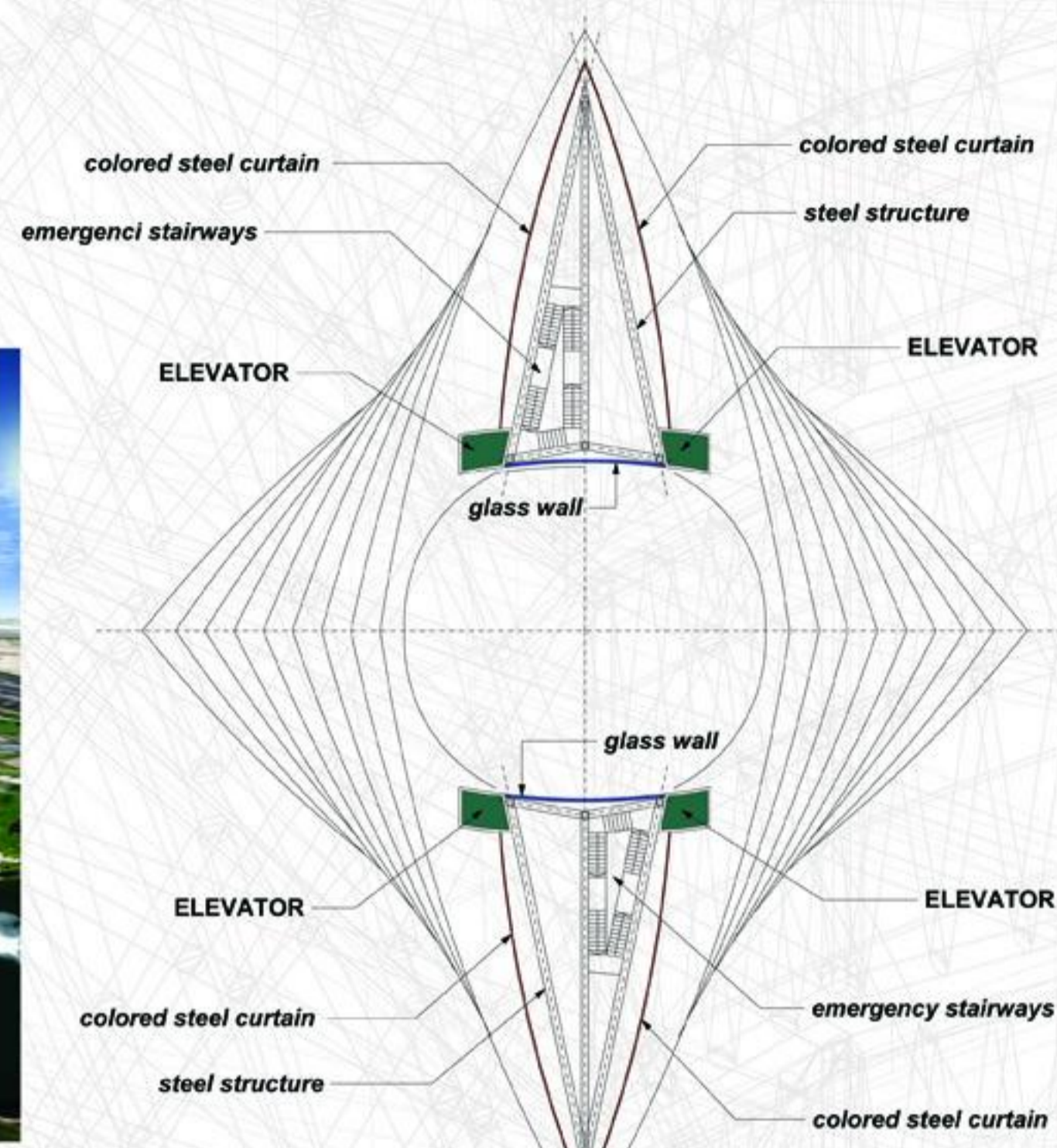
middle level plan
