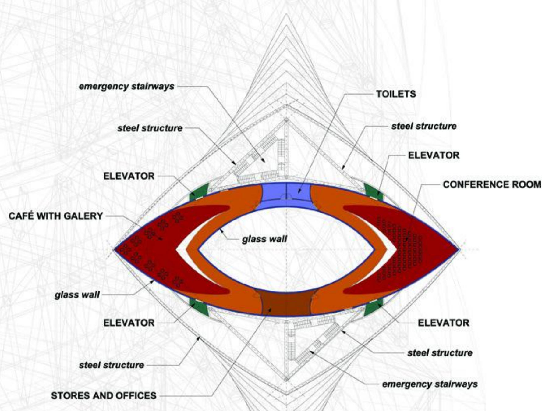
top level plan
