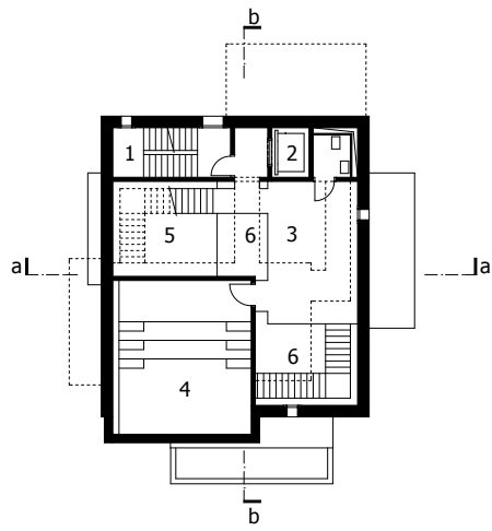
Harmadik emeleti alaprajz - Third floor plan M 1:400 - Scale 1:400
