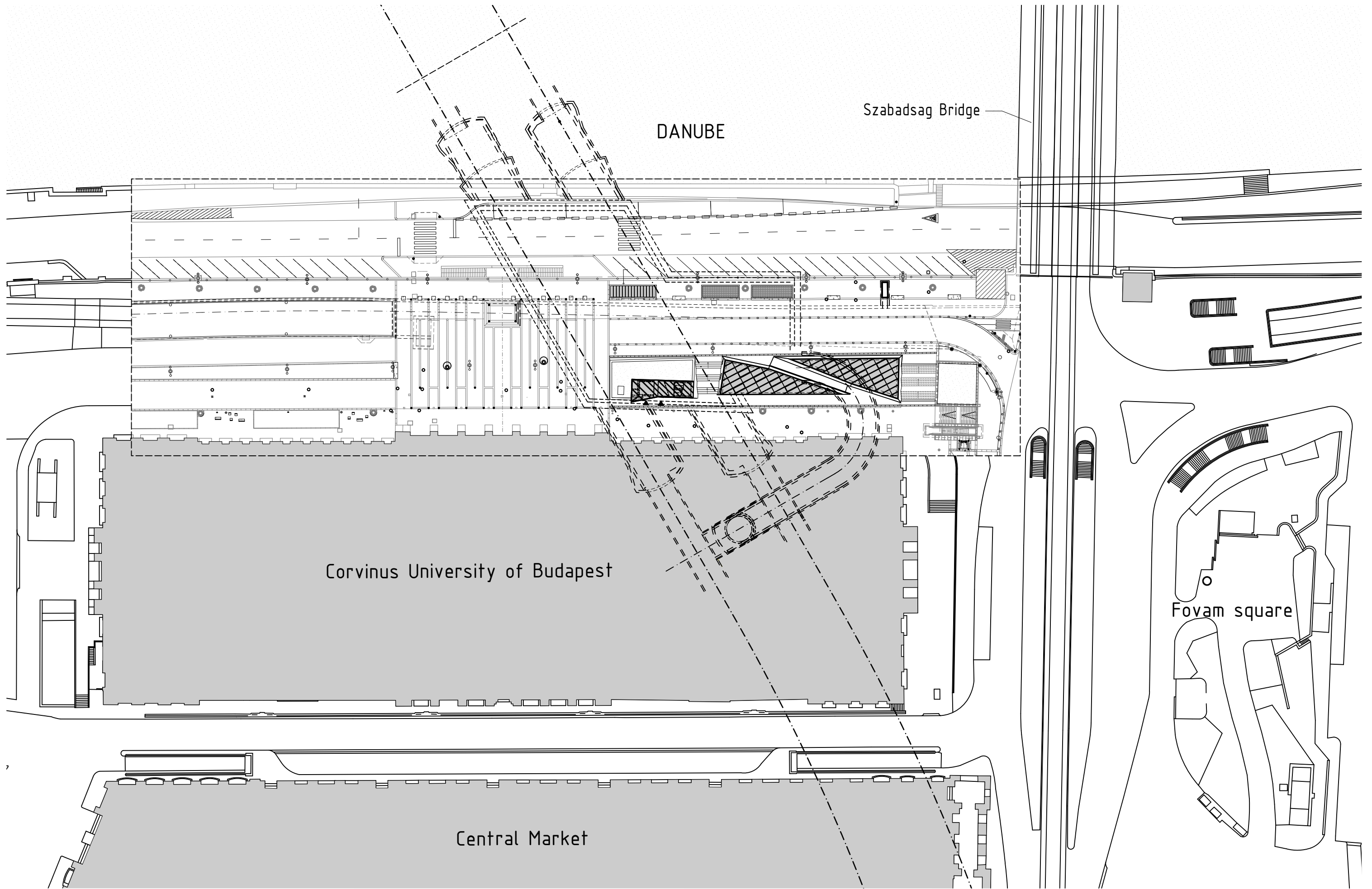
site plan
