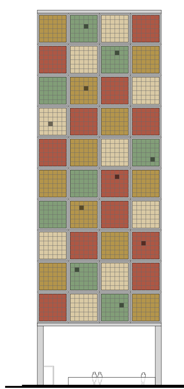
West elevation
