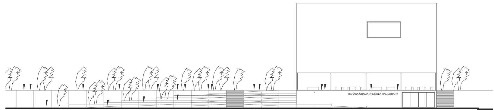
West elevation
