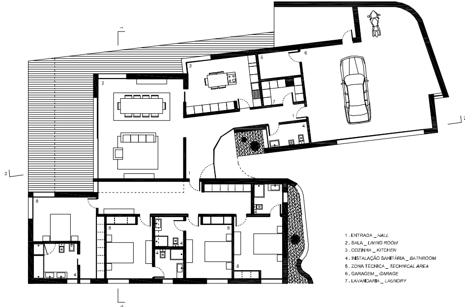
\\ PLANTA PISO 0 _ GROUND LEVEL PLAN
