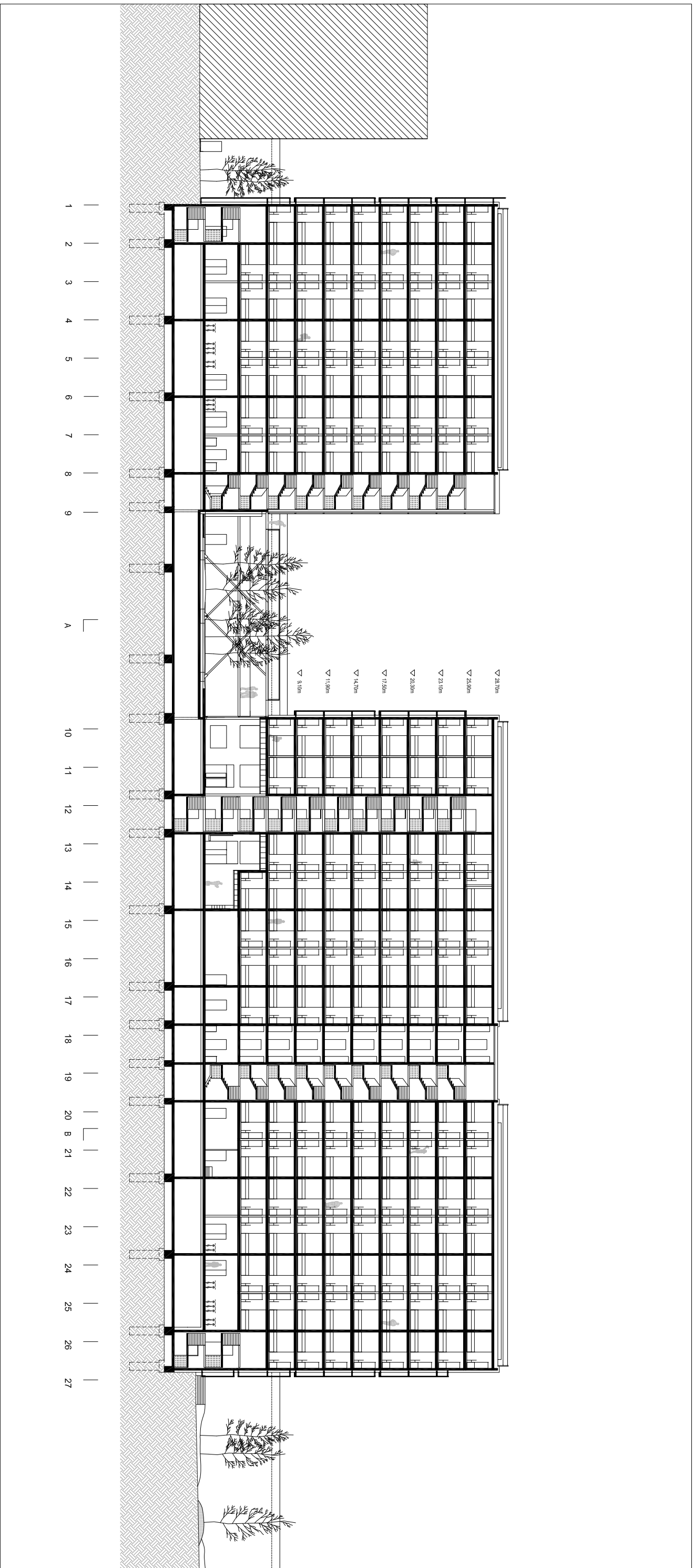
SECTION C 0 5 10m
