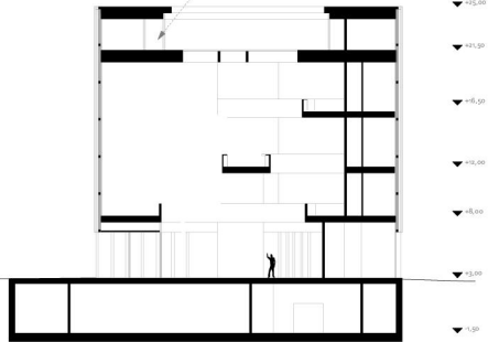
D - D SECTION 1:200
