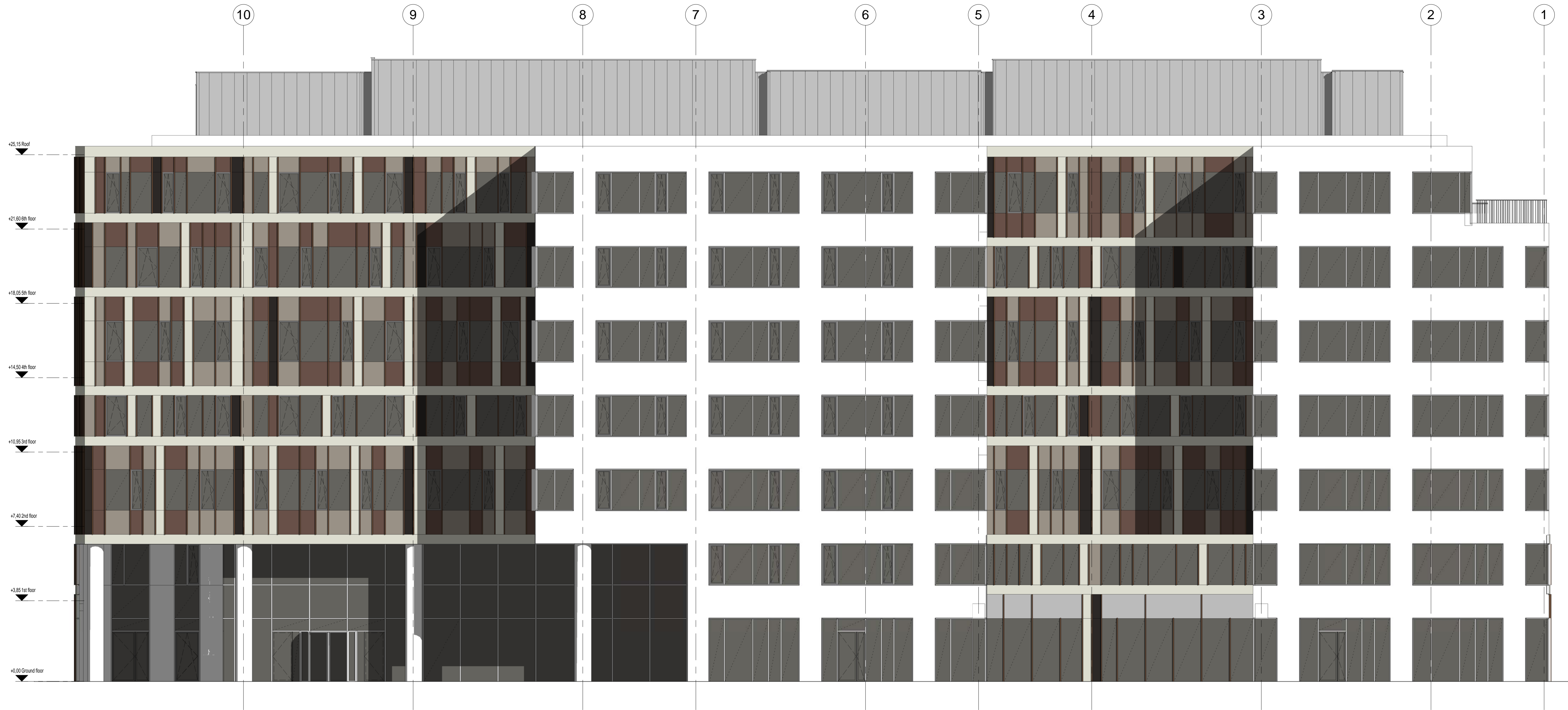
Promenade Facade M I Scale 1 : 100
