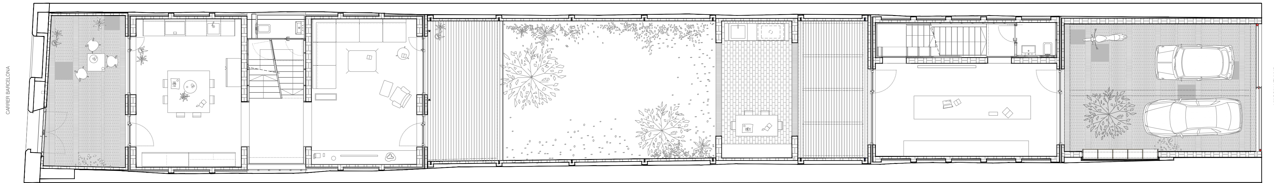
PLANTA BAIXA / GROUND FLOOR
